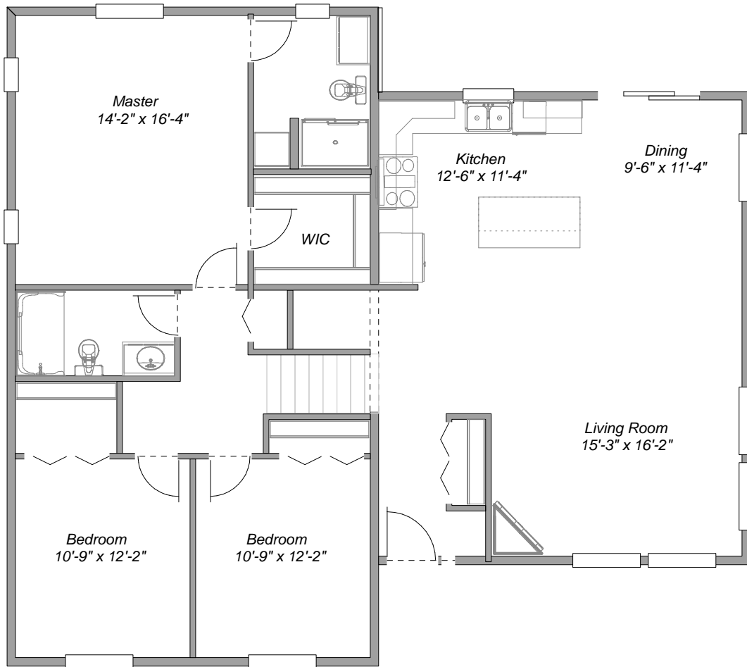
PLAN CU-S-26
