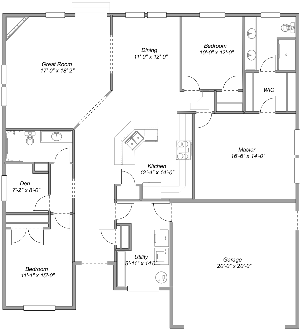
CI-R-5 MAIN FLOOR PLAN
